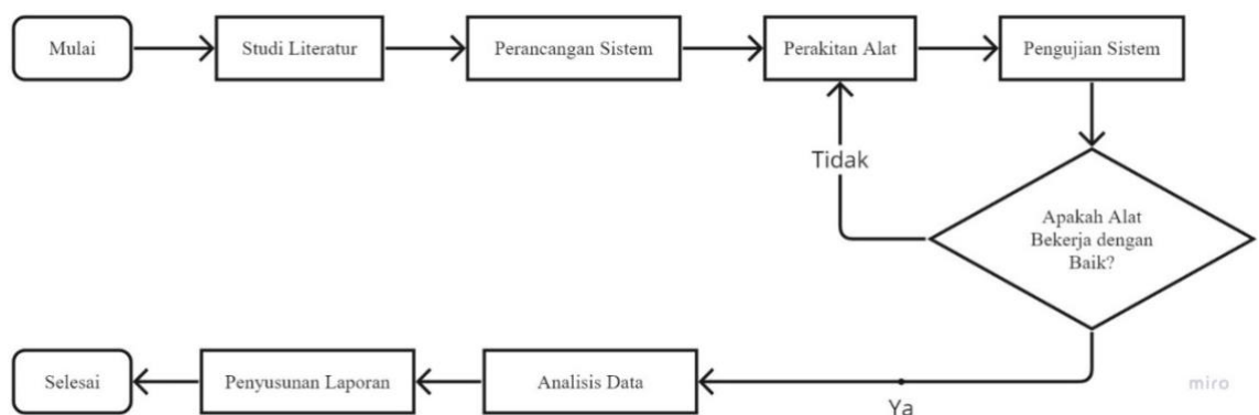
Figure 1. Flowchart Methodology
